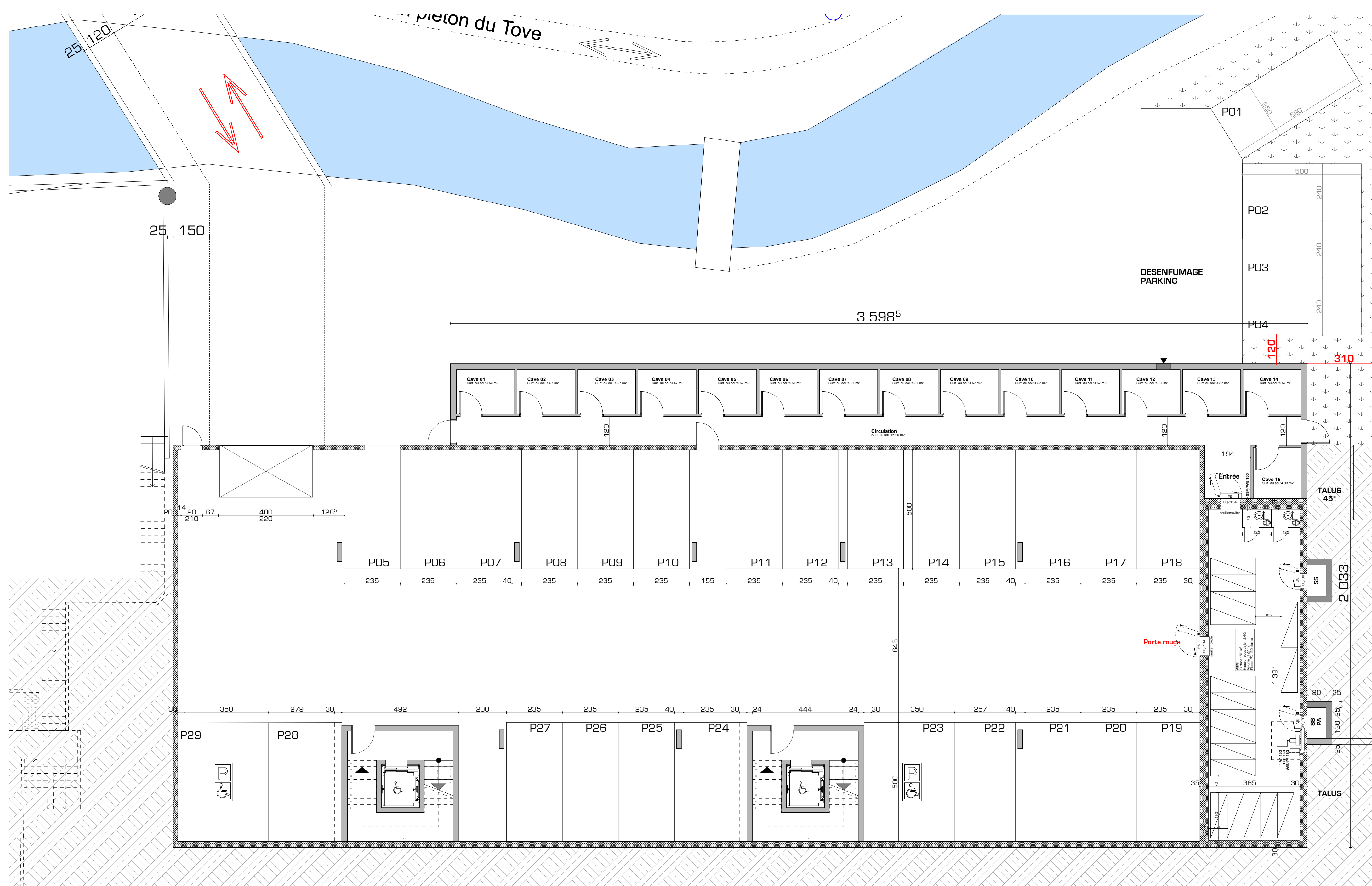
REZ ECH. 1:100
